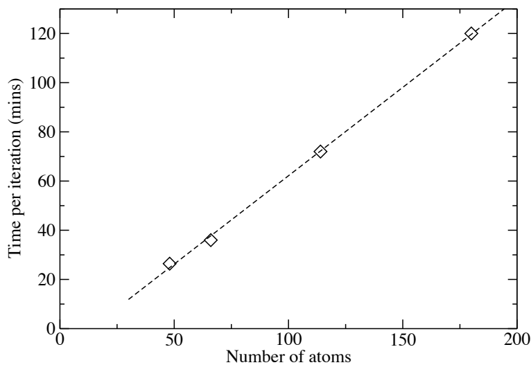
Figure 3. Scaling of the time per iteration against system-size represented by the number of atoms in the cluster
